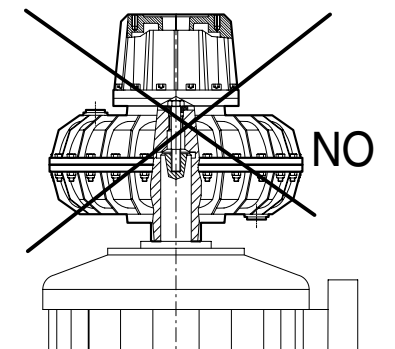
VERTICAL SHAFT WITH UPWARD DELAY CHAMBER
