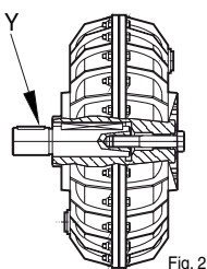
ROTOFLUID ALFA K-Y with pin shaft
